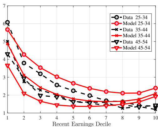
(C) EE-rate: Model vs. SIPP
